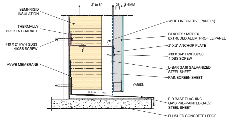
EXTRUDED ALUM. PROFILE PANEL
