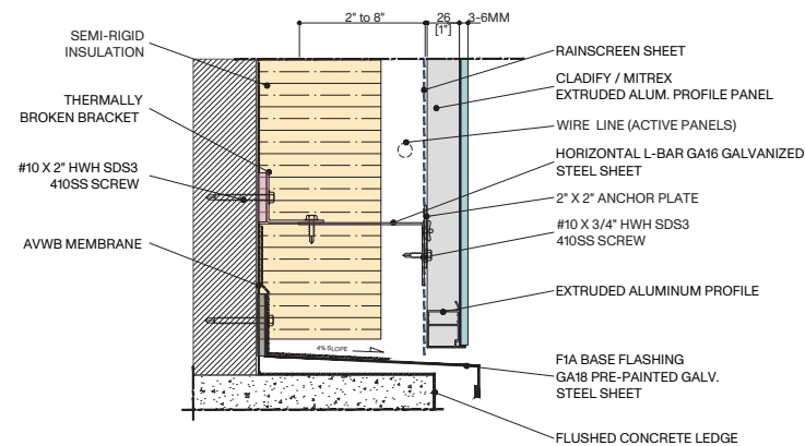
EXTRUDED ALUM. PROFILE PANEL
