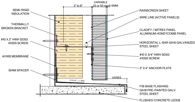
ALUMINUM HONEYCOMB PANEL
