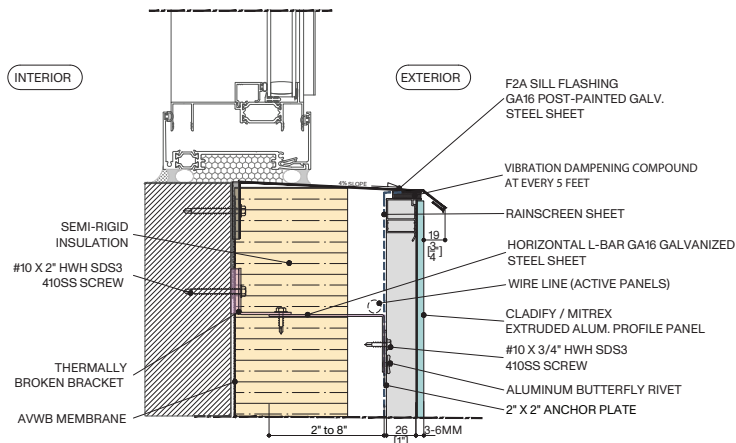
EXTRUDED ALUM. PROFILE PANEL
