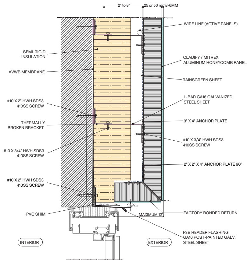
ALUMINUM HONEYCOMB PANEL PRE-ASSEMBLED RETURN PANEL (ANCHOR PLATE - SIDE CONNECTION)
