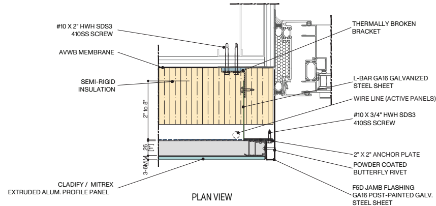
EXTRUDED ALUM. PROFILE PANEL
