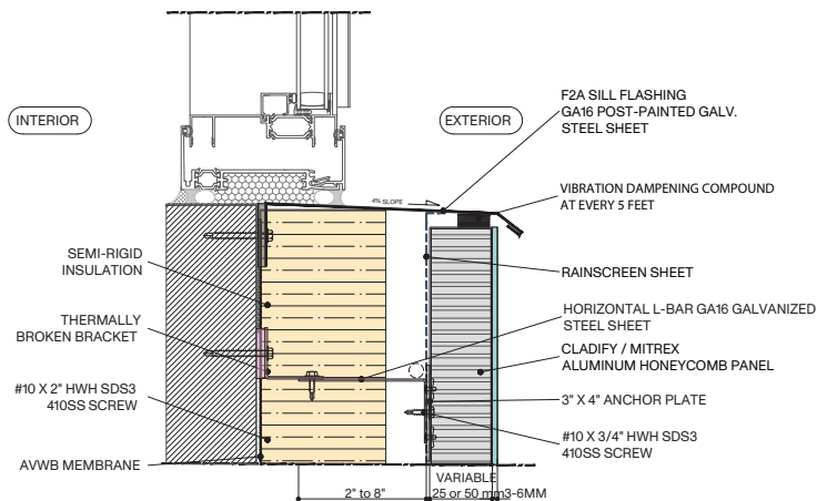
ALUMINUM HONEYCOMB PANEL
