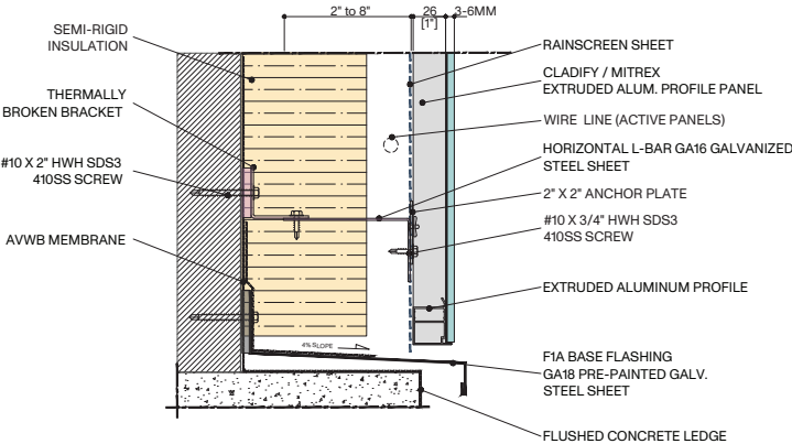
EXTRUDED ALUM. PROFILE PANEL
