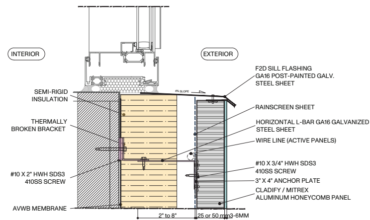
ALUMINUM HONEYCOMB PANEL
