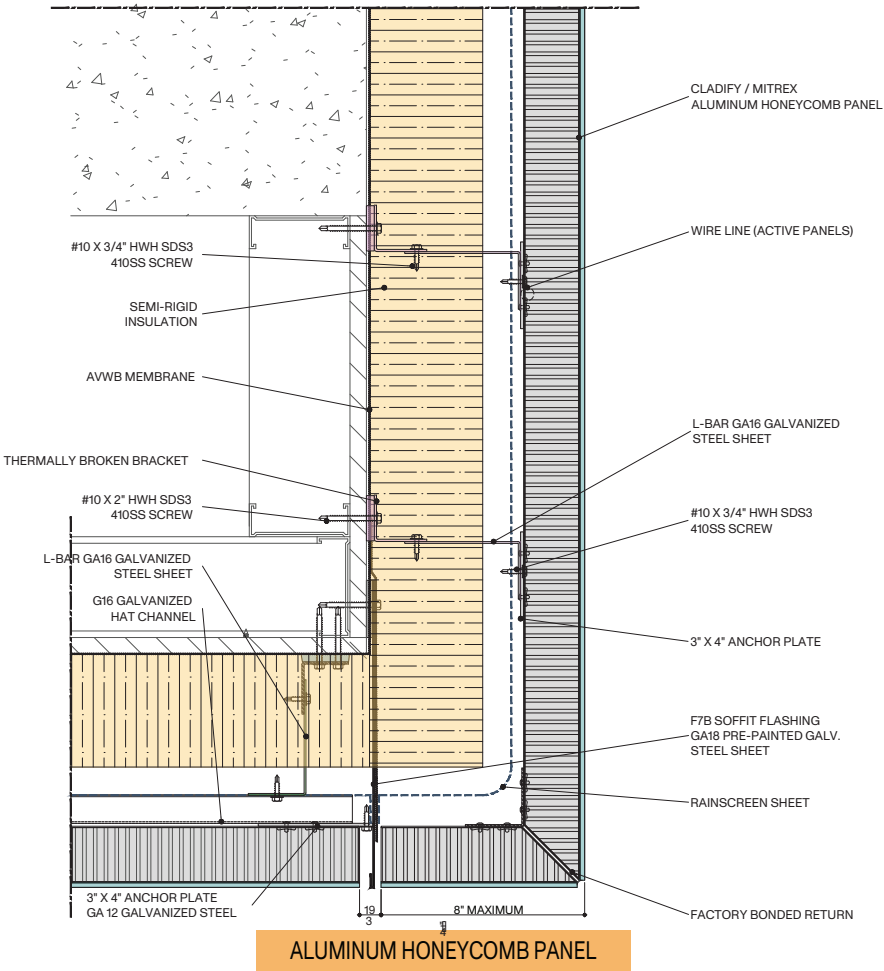
PRE-ASSEMBLED SOFFIT RETURN
