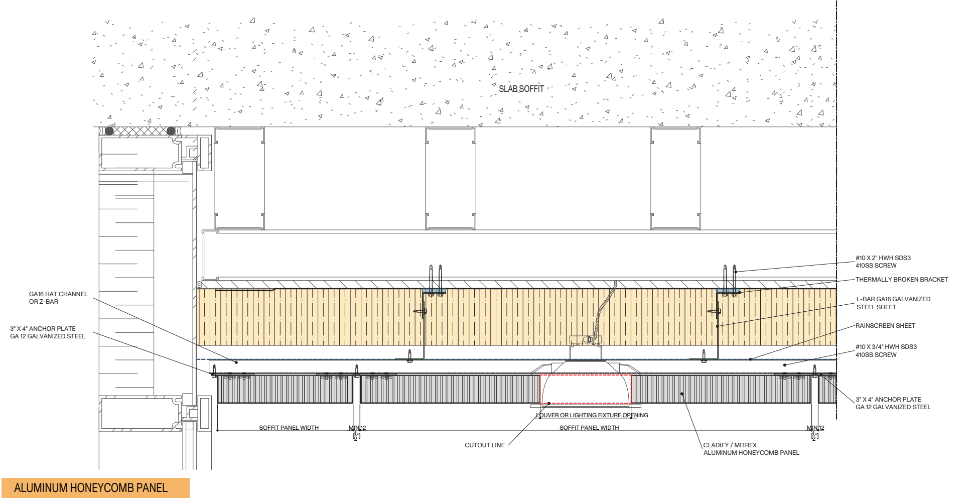
SOFFIT PANEL CUTOUT
