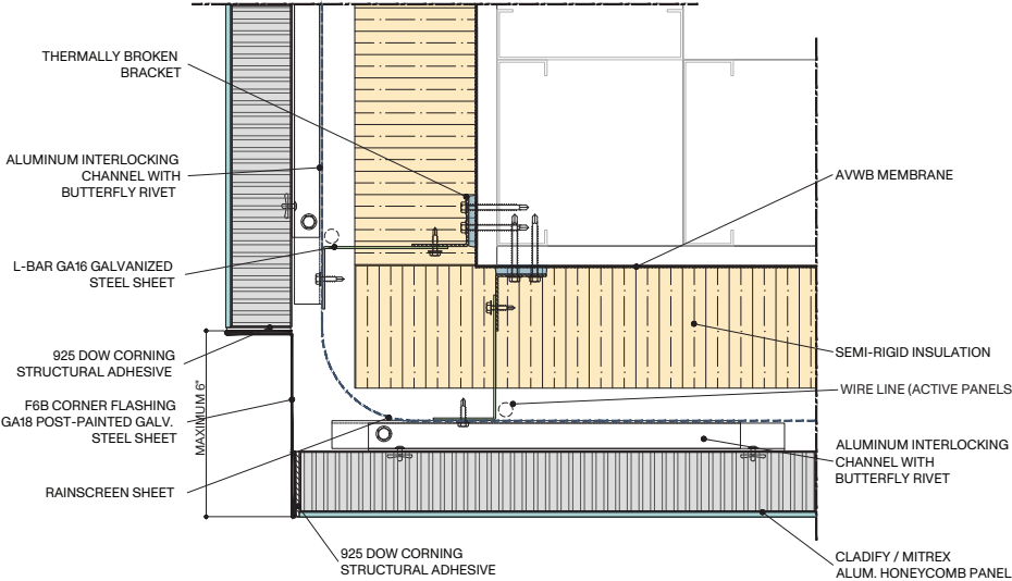
PLAN VIEW (OPTION 2)
