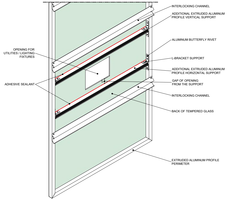
REAR VIEW ISOMETRIC
