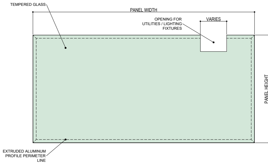
FRONT ELEVATION
