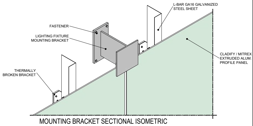
INSERTION OF MOUNTING BRACKET IN BETWEEN 2 PANELS
