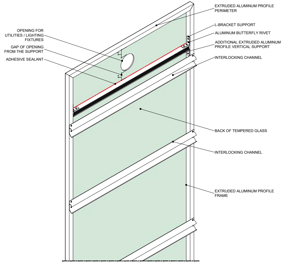
REAR VIEW ISOMETRIC
